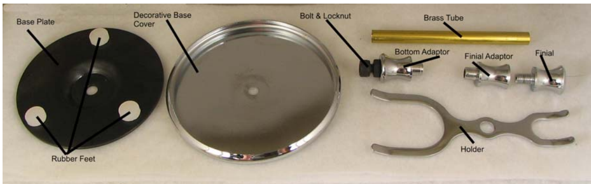
Parts Diagram
